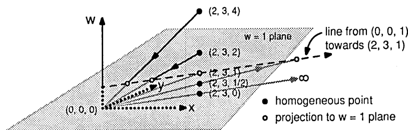
Figure 3: projection to the w = 1 plane.
