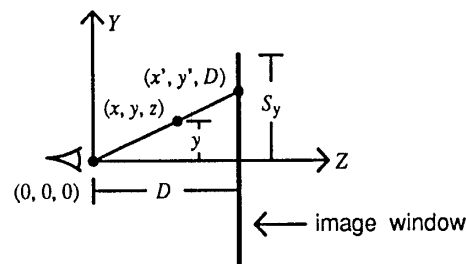
Figure 5: the perspective projection
