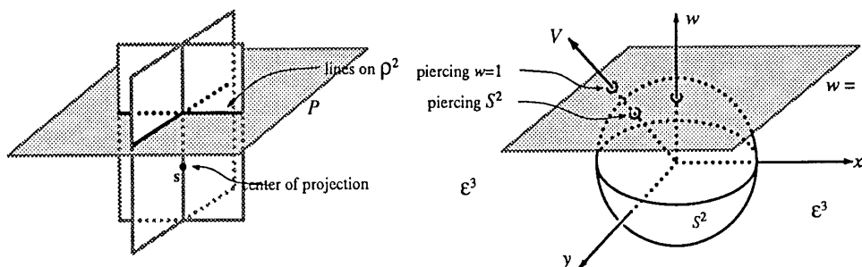
Figure 2: the projective plane.
