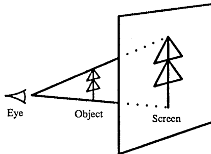
Figure 4: perspective projection onto the raster-screen.
