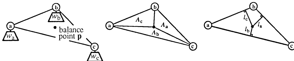
Figure 1: barycentric and Plücker coordinates.
