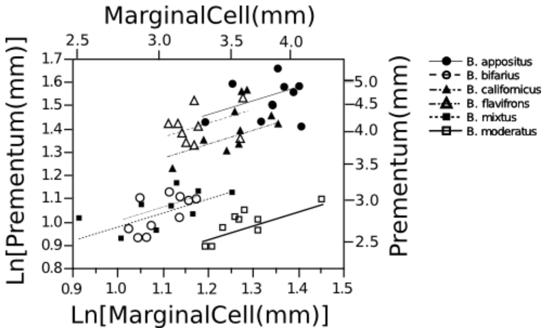
Figure 2.3 Prediction of prementum length ( \ln[\text{mm}] ) from marginal cell length ( \ln[\text{mm}] ) and bee species ( N = F_{6,50} = 88.21 , p < 0.0001 , R^2=0.91 ).
