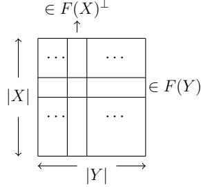
Figure 2.3: Finiteness matrix
