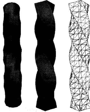
Figure 6. Twisted rod of intersecting planes, right images include CSG post-processing
