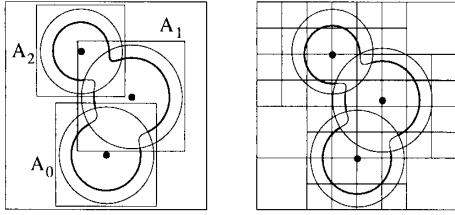
Figure 7. Space subdivision vs. bounding volume subdivision
