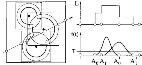
Figure 8. Interval creation through bounding boxes ray tracing
