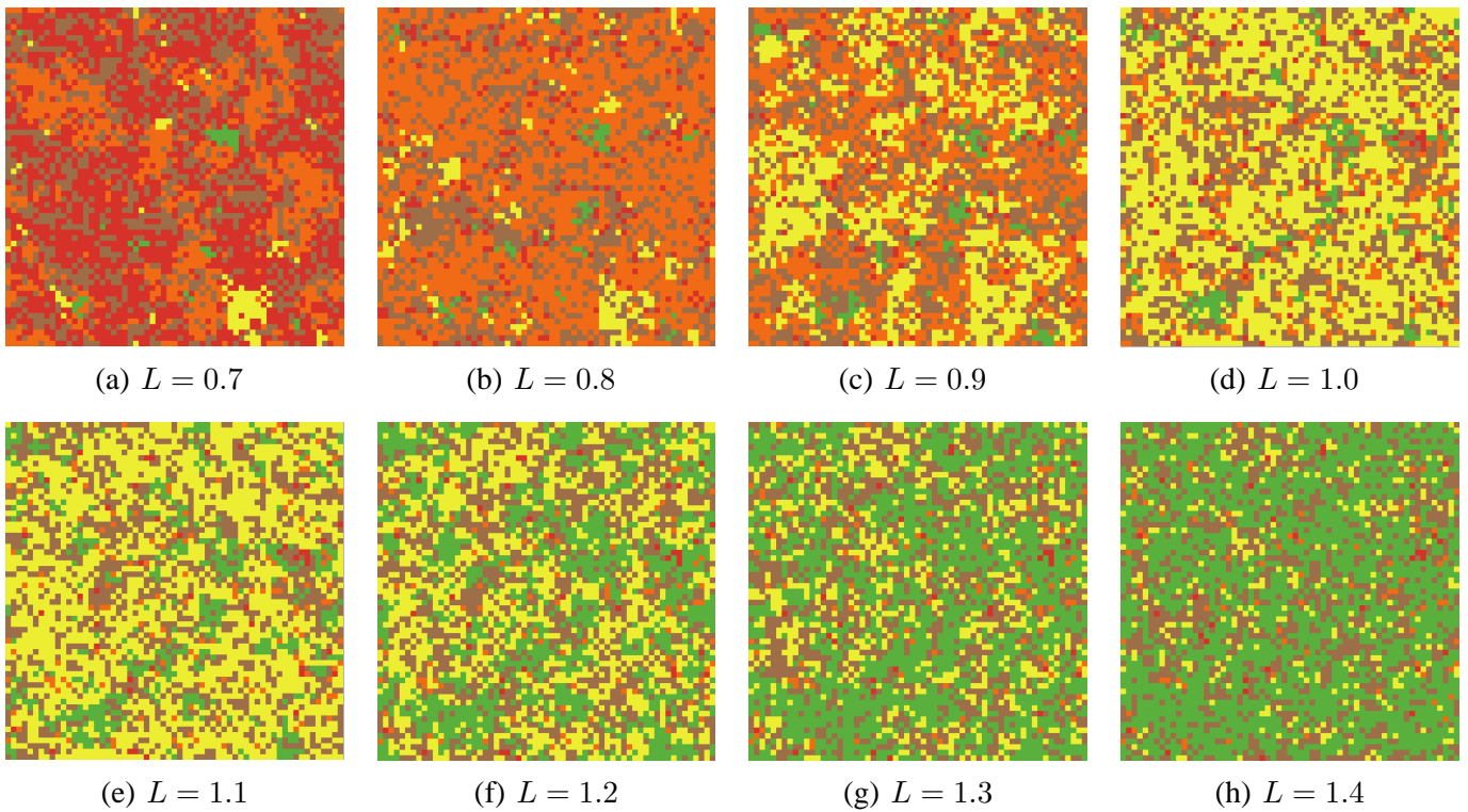
Fig. 7. Effects of Solar Luminosity ( L ) on Four Species Daisy World
