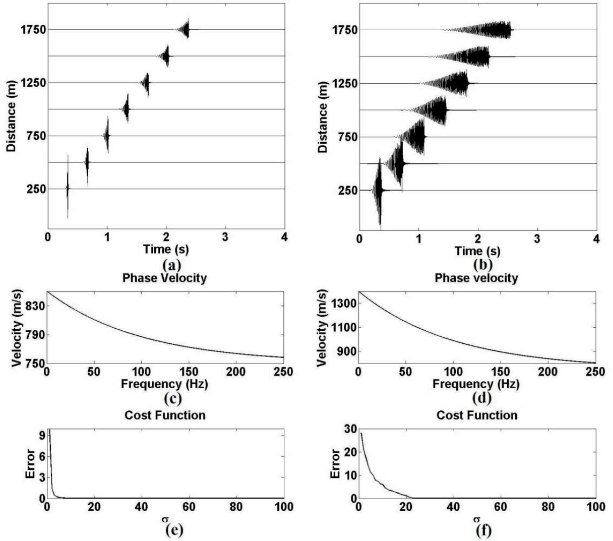
Figure 2.8 (a) and (b) Two different dispersed data sets; (c) and (d) the phase velocities for (a) and (b), respectively; (e) and (f) the cost functions for (a) and (b), respectively.
