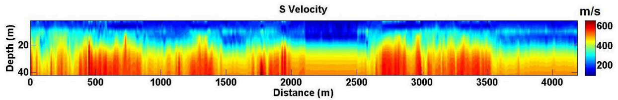
Figure 4.13 The S-wave velocity model for the Hussar data obtained from the phase velocity in Figure 4.12.
