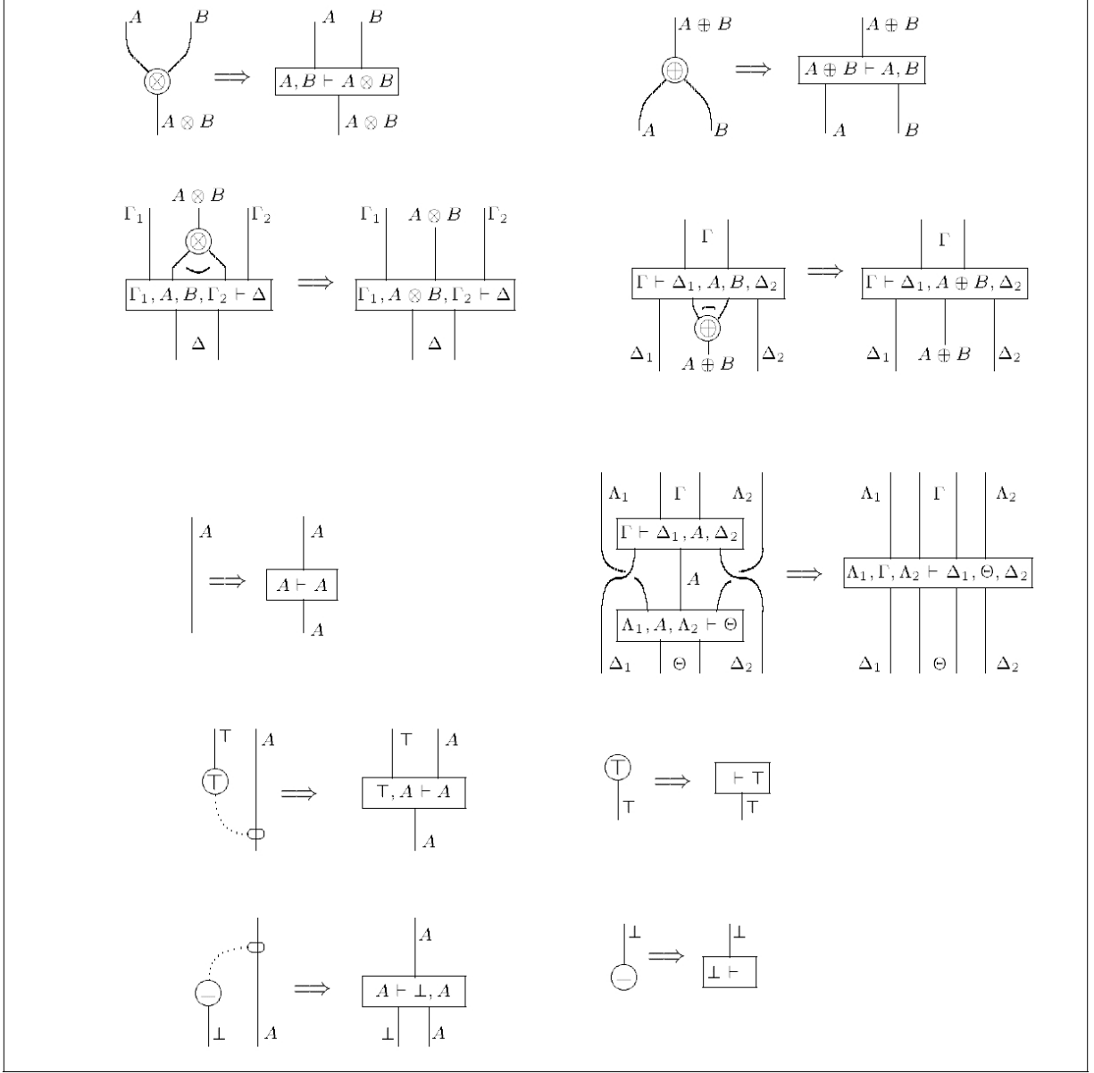
Figure 2.4: Sequentialization Procedure
