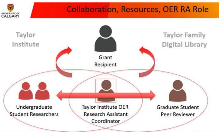
Figure 1: Grant Model
