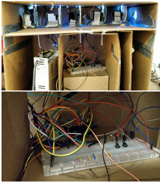
Figure 5: The electronic components of the physicalization (Figure 4), and the interface to cycle through years. Note the same RAMPS board and power supply as the CNC plotter.
